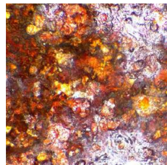
Figure 1. Detailed surface morphology of uncovered steel sample after 500 cycles.
